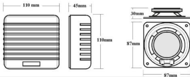
Diagrammatic layout
